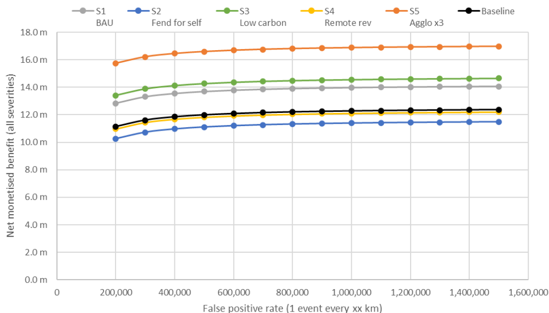
Figure 43: Comparison of the net monetised effect of the AEB max variant (Using updated data from CCTV and telematics analysis and adjusted for empty buses)
