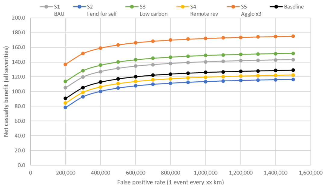
Figure 42: Comparison of the net casualty effect of the AEB max variant (Using updated data from CCTV and telematics analysis and adjusted for empty buses)
