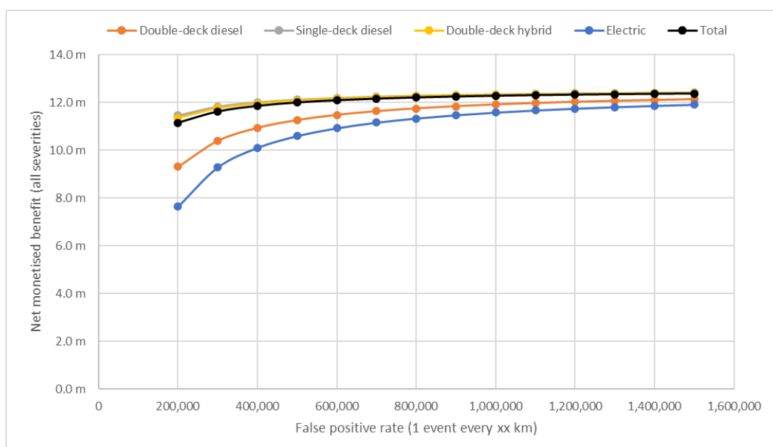
Figure 57: Net monetised casualty effect (all casualty types) by false positive rate for different drivetrains – AEB max
