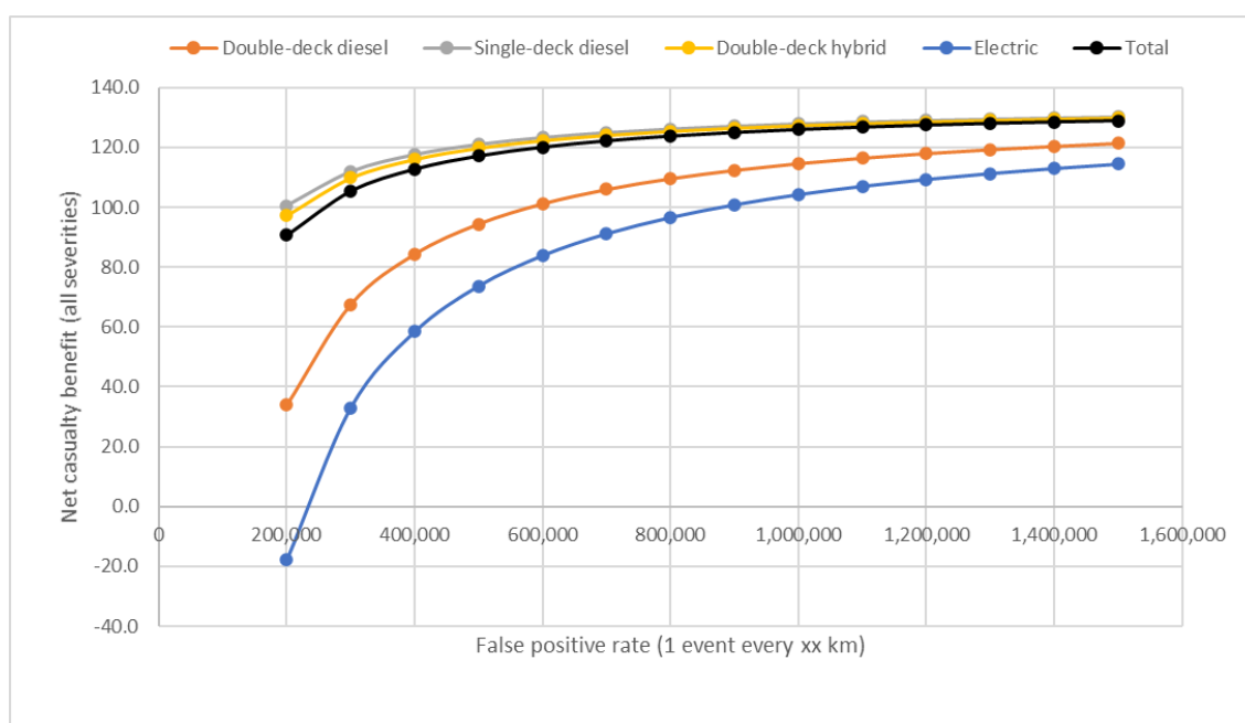
Figure 56: Net casualty effect (all casualty types) by false positive rate for different drivetrains – AEB max
