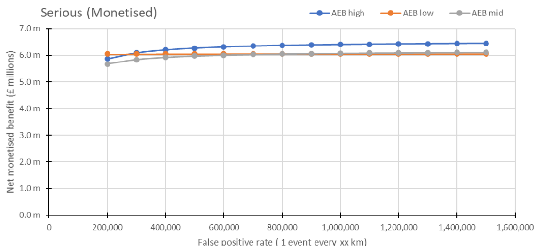
Figure 33: The effect of false positive rate on the annual net monetised benefit of each candidate AEB system (central prediction) for serious casualties only (Using updated data from CCTV and telematics analysis and adjusted for empty buses)
