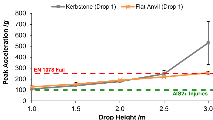
Figure 2: Mean peak linear headform accelerations compared to drop height for impacts against flat and kerbstone anvils during the first impact (Drop 1) only. The 250 g threshold line represents the pass/fail criterion specified by EN 1078, whilst the 100 g threshold line represents the AIS2+ injury criteria specified by Newman (1980) (BSI, 2012). Error bars represent the 95% confidence intervals of the mean.
