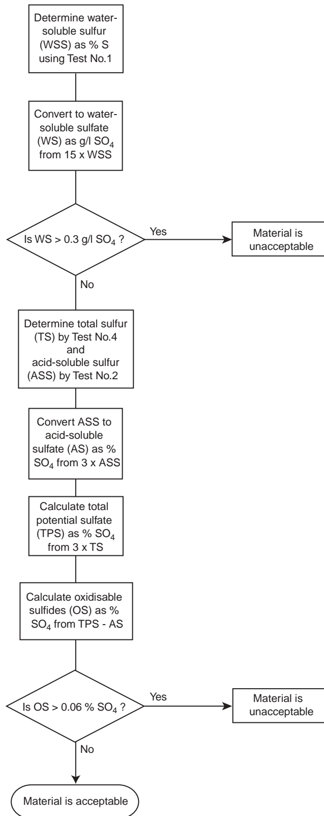
Figure 8.1 Flow chart assessment of structural backfill to galvanised steel elements
