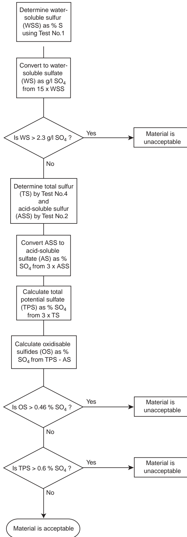
Figure 8.2 Flow chart assessment of fill placed within 500mm of concrete or cement bound materials
